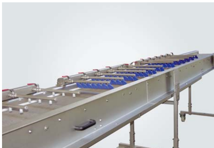
Integrated EBG system with conveyor belt, air knife and strand pelletizer
